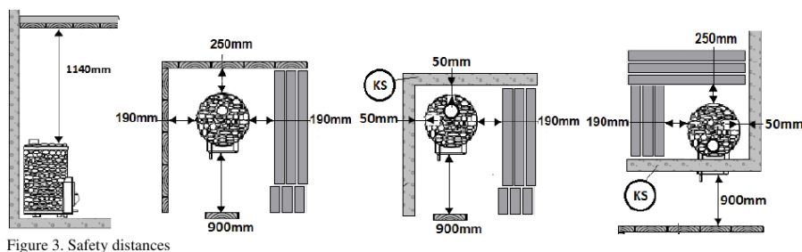
Figure 3. Safety distances
